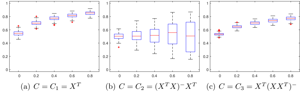
Figure 1: Boxplots of the probabilities computed from (9), for different values of \rho , taken over 250 simulated data sets with N = 20 .
