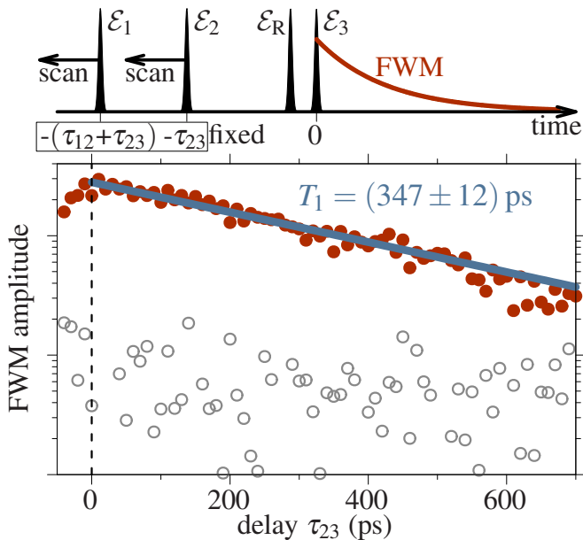
FIG. 2. Top: Three-pulse sequence employed to measure the trion population dynamics. \mathcal{E}_1 and \mathcal{E}_2 , having a delay of \tau_{12} = 20 ps, create the trion population and are jointly advanced in time, such that the FWM triggered by \mathcal{E}_3 probes the population decay via the \tau_{23} dependence. Bottom: Measurement yielding the exciton lifetime T_1 = (347 \pm 12) ps. The noise level is indicated by open circles.
