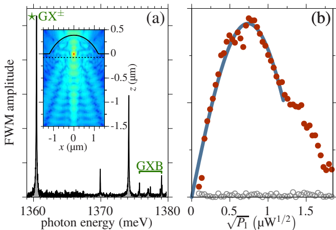
FIG. 1. (a) Spectrally-resolved FWM amplitude generated by a few QD excitons embedded in a lens structure. The targeted QD trion ( GX^\pm ) is labeled with the green \star . The horizontal bar indicates a neutral exciton-biexciton system (GXB) in a QD located at the lens periphery. Inset: Calculated distribution of the near-field intensity for the QD-lens structure. The semiconductor-air interface is shown by the solid black line and the DBR starts below the dashed line. (b) Spectrally-integrated FWM amplitude of a trion in the target QD as a function of the pulse area \theta_1 \propto \sqrt{P_1} of \mathcal{E}_1 . The blue line shows the fit to the expected |\sin(\theta_1/2)| amplitude dependence of the FWM.
