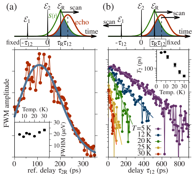
FIG. 3. (a) Top: Two-pulse sequence applied to probe the echo profile. Bottom: Integrated FWM amplitude versus \tau_{2R} at 5K revealing the Gaussian echo with a temporal width yielding \sigma ; the theoretical fit is given by the solid line. Inset: Inhomogeneous broadening \sqrt{8 \ln(2)}\sigma retrieved from the echo temporal width for different temperatures. (b) Top: Two-pulse sequence applied to probe the trion dephasing. Bottom: Measured FWM amplitude as function of the delay \tau_{12} , yielding coherence dynamics for different temperatures; theoretical fits as solid lines. Inset: Dephasing time T_2 as a function of temperature.
