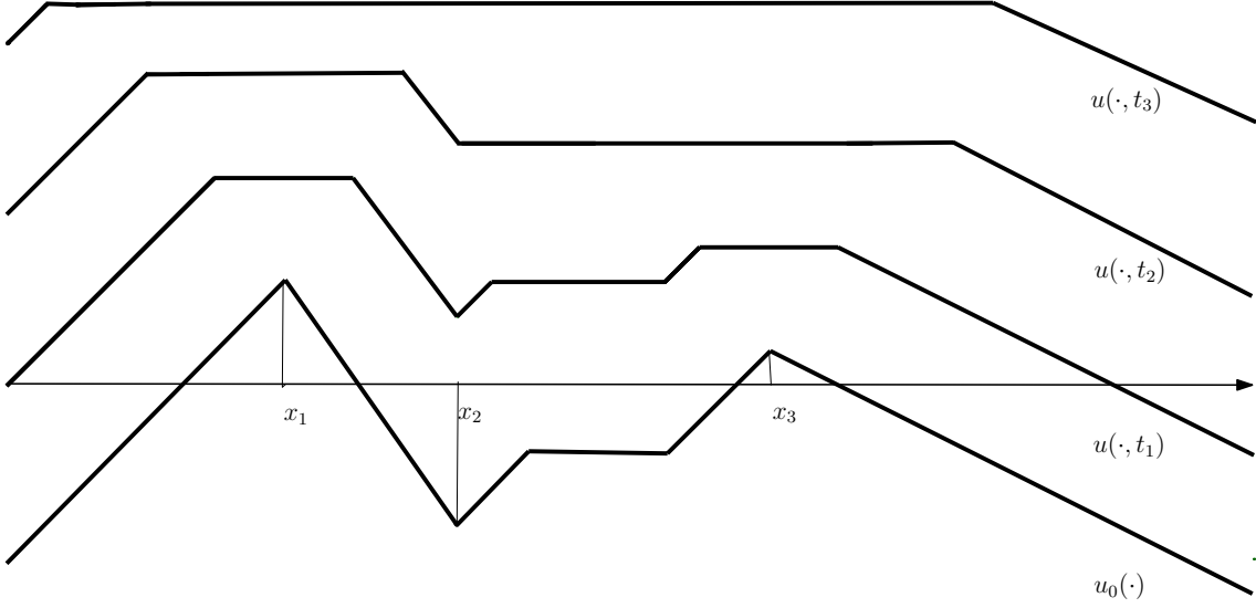
Figure 1: Example of the solution (44) selected as \varepsilon \rightarrow 0 , with initial datum u_0 .
