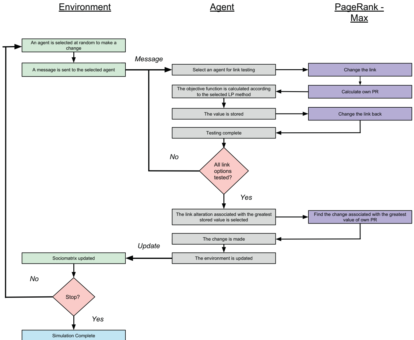
Fig. 5. Updated simulation logic describing the process of the PR-Max method.
