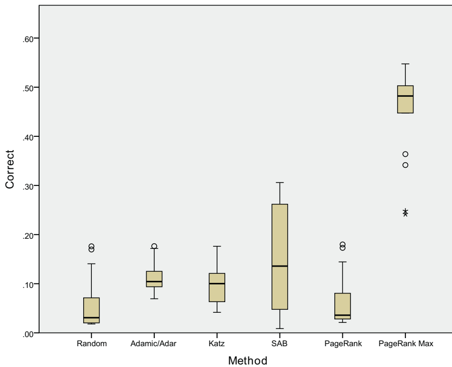
Fig. 7. Box plot of correct prediction proportions for each method at T_3 . Whiskers extend 1.5 times the height of the box, with circular points indicating outliers. Starred points indicate extreme outliers.
