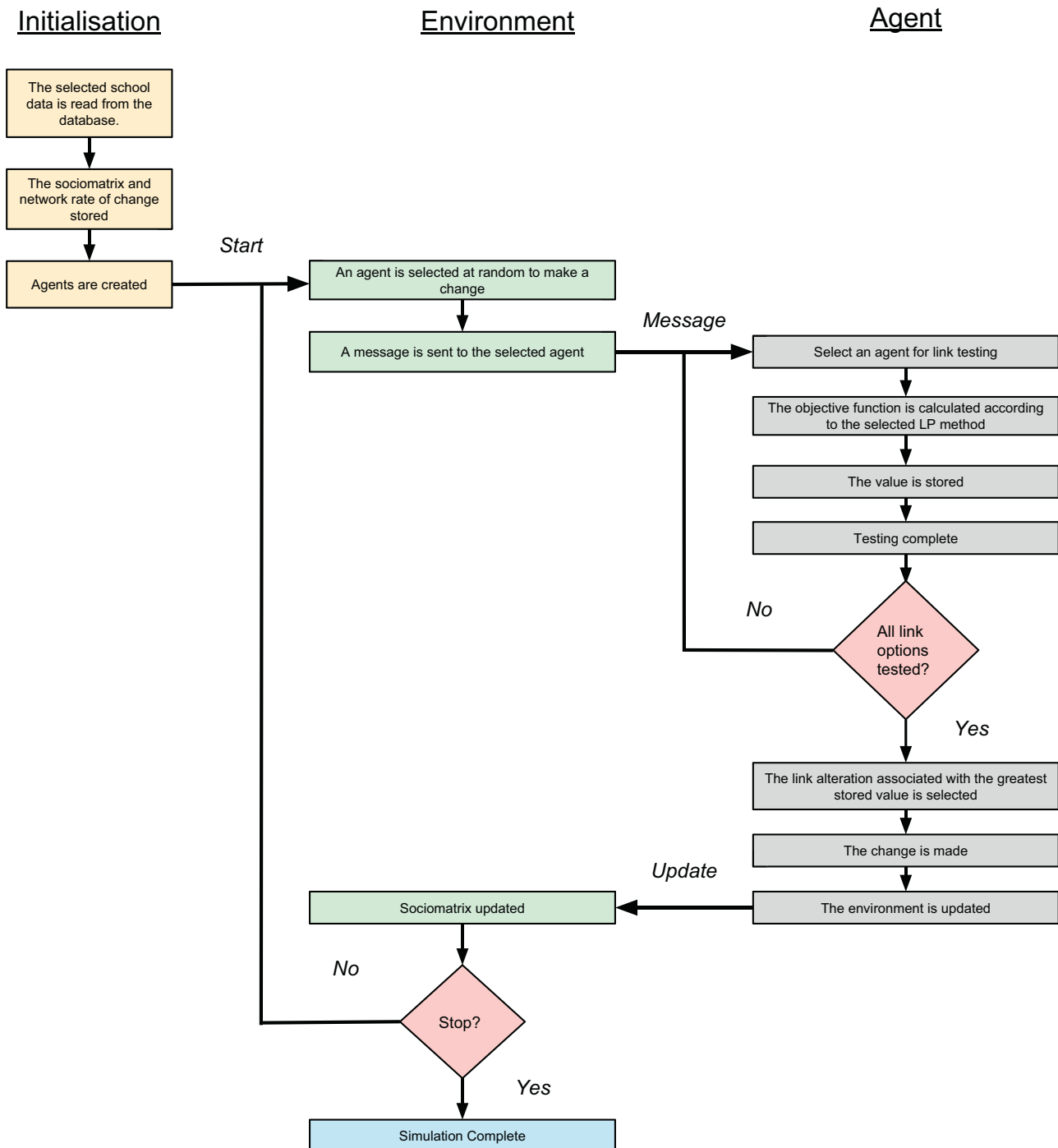
Fig. 4. Simulation logic describing the timing and agent-based decisions.
