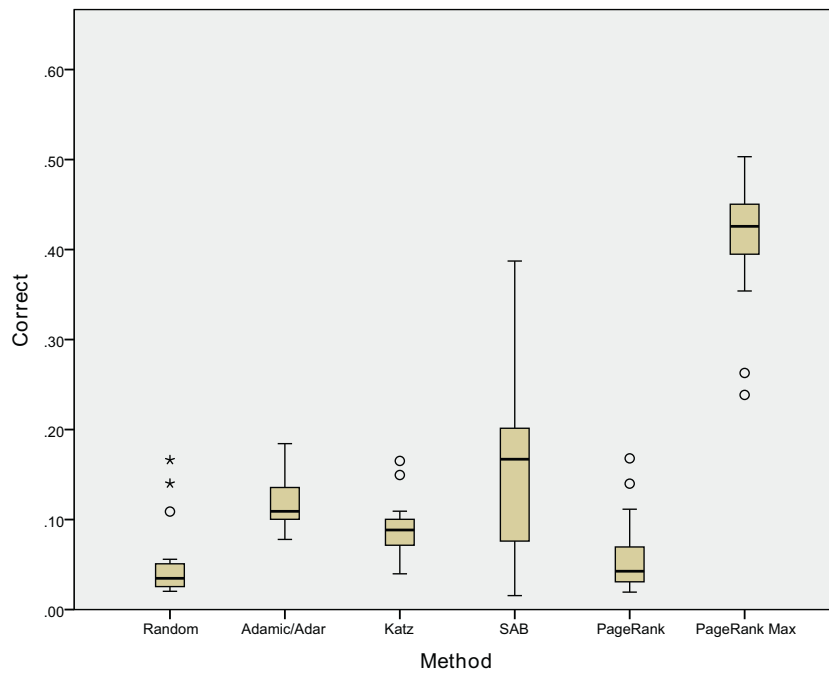
Fig. 6. Box plot of correct prediction proportions for each method at T_2 . Whiskers extend 1.5 times the height of the box, with circular points indicating outliers. Starred points indicate extreme outliers.
