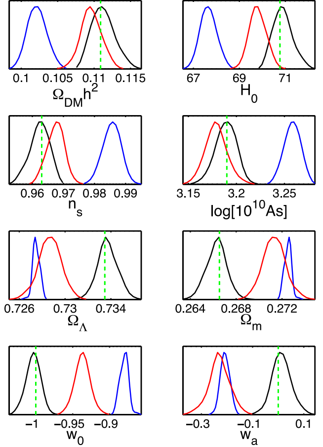
Figure 4. Same as Fig. 3 but for the w_0 w_a CDM model, where the two parameters ( w_0 , w_a ) are added to the fit.
