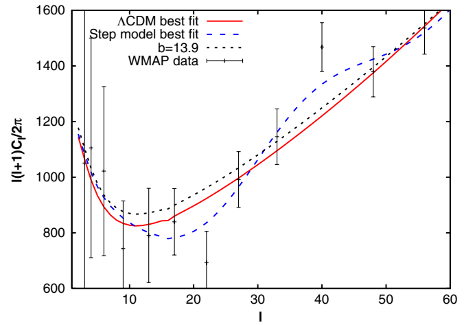
FIG. 5 (color online). (Top) CMB anisotropy spectrum for the \Lambda CDM (red solid line) and generalized step model (blue long dashed line) best fits, and for a step model with b = 13.9 (black short dashed line), compared with the WMAP7 data. (Bottom) Zoom of the region \ell \leq 60 , showing the improved fit of the step model.
