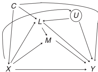
Figure 3. Causal diagram for exposure X , mediator M , outcome Y , intermediate confounder L , and unmeasured intermediate L - Y confounder U . The circle around U indicates that it is unmeasured.
