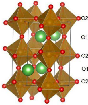
Figure 1. Orthorhombic form of LaFeO 3 ; lanthanum are shown in green, iron in gold and oxygen in red. The two oxygen environments; O1 and O2 are shown to the right of the structure.
