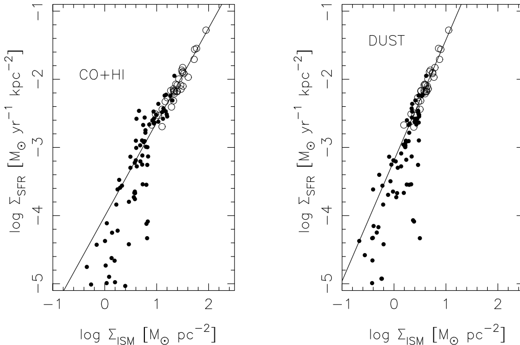
Fig. 2. The same as Fig. 1 but for M100. For this galaxy the open circles show points within 100 arcsec of the centre of the galaxy, the region in which the surface-density of the molecular gas is greater than that of the atomic gas.
