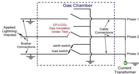
Figure 3. Standard lightning impulse test connections for Ringmaster and Fluokit switch disconnectors.
