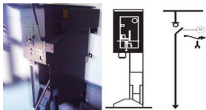
Figure 1. Ringmaster SE6 switch disconnector [14].
