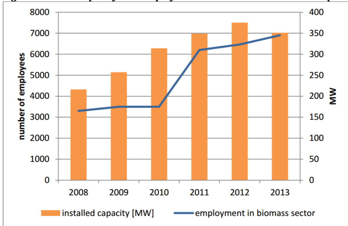
Fig. 6: Installed capacity and employment in biomass in the Czech Republic (2008-2013)
