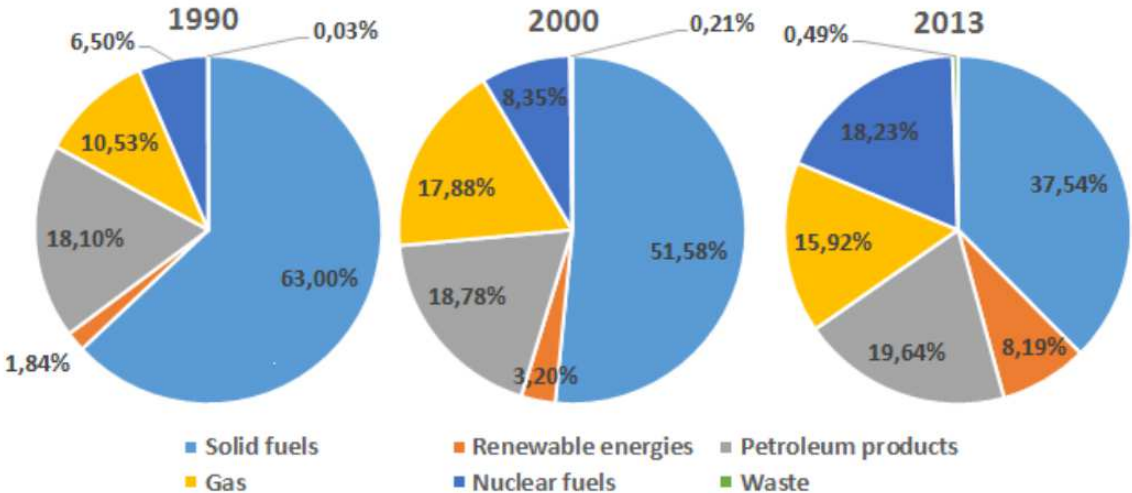
Fig. 1: Gross domestic energy consumption in the Czech Republic
