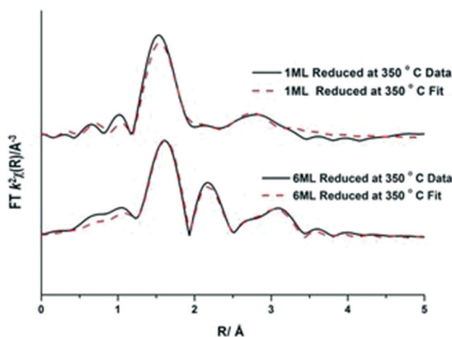
Fig. 10 Magnitude component of the k^2 weighted Fourier transform for the EXAFS data of the 1 and 6 ML MoO x /Fe 2 O 3 catalyst reduced (procedure as in Fig. 9), and the associated simulated fit performed in Artemis.
