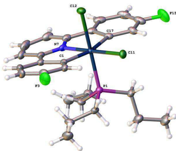
Figure 5: The solid-state structure of 2c(c) , thermal ellipsoids drawn at 50% probability level. Selected bond lengths (Å) and angles (°): Pt1-P1 2.2944(11); Pt1-Cl2 2.4116(10); Pt1-C1 2.069(4); Pt1-C17 2.083(4); Pt1-N7 1.981(3); Pt1-Cl1 2.3282(10); C11-N7 1.352(6); C7-N7 1.364(6); P1-Pt1-Cl2 175.49(4); P1-Pt1-Cl1 85.53(4); C1-Pt1-P1 91.42(11); C1-Pt1-Cl2 85.48(10); C1-Pt1-C17 162.32(17); C1-Pt1-Cl1 97.86(12); C17-Pt1-P1 93.94(11); C17-Pt1-Cl2 89.98(11); C17-Pt1-Cl1 99.34(13); N7-Pt1-P1 95.28(10); N7-Pt1-Cl2 87.51(10); N7-Pt1-C1 81.56(15); N7-Pt1-C17 81.18(16); N7-Pt1-Cl1 179.01(10); Cl1-Pt1-Cl2 91.65(4).
