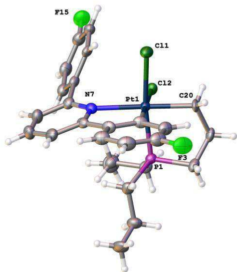
Figure 6: The solid-state structure of 6c(e) , thermal ellipsoids drawn at 50% probability level. Selected bond lengths (Å) and angles (°): Pt1-Cl1 2.3953(15); Pt1-Cl2 2.4072(16); Pt1-C1 2.030(7); Pt1-N7 2.246(5); Pt1-P1 2.2650(15); Pt1-C20 2.076(6); C18-P1 1.828(6); C18-C19 1.480(16); C11-Pt1-Cl2 91.68(6); C1-Pt1-C11 89.54(19); C1-Pt1-Cl2 178.72(19); C1-Pt1-N7 79.7(3); C1-Pt1-P1 87.46(19); C1-Pt1-C20 96.2(3); N7-Pt1-Cl1 91.74(14); N7-Pt1-Cl2 100.66(15); N7-Pt1-P1 95.20(14); P1-Pt1-Cl1 171.83(5); P1-Pt1-Cl2 91.29(6); C20-Pt1-C11 87.93(19); C20-Pt1-Cl2 83.4(2); C20-Pt1-N7 175.9(3); C20-Pt1-P1 84.84(19).
