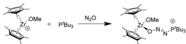
Figure 3. Zr(IV) cations used in this work. The [B(C 6 F 5 ) 4 ] - counterions has been omitted for clarity.
