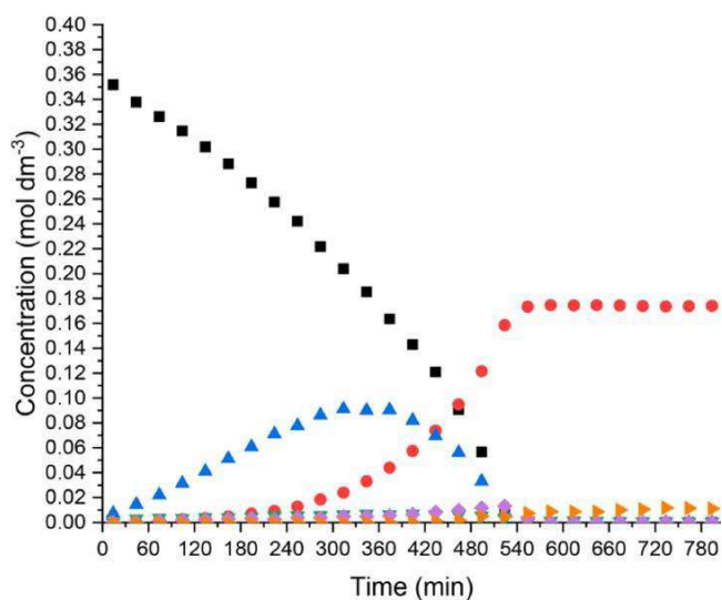
Figure 6. Reaction of 1a with \text{Me}_2\text{NH}\cdot\text{BH}_3 (25 °C, PhBr- d_5 , 14 h): (black ■) \text{Me}_2\text{NH}\cdot\text{BH}_3 ; (red ●) [\text{Me}_2\text{N}-\text{BH}_2]_2 ; (blue▲) \text{Me}_2\text{NH}-\text{BH}_2-\text{Me}_2\text{N}-\text{BH}_3 ; (purple ) \text{Me}_2\text{N}=\text{BH}_2 ; (green ▼) \text{Me}_2\text{N}(\text{B}_2\text{H}_5) ; (orange triangles) \text{HB}(\text{NMe}_2)_2 .
