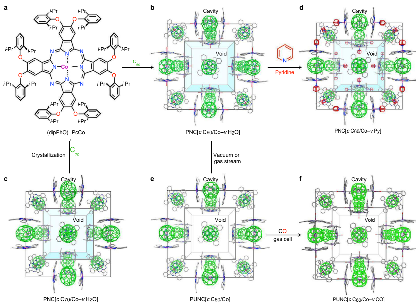
Fig. 1 | The crystal structures of the fullerene-containing PNCs. a , The molecular structure of (dipPhO) 8 PcCo. b,c , The fullerene-stabilized PNC[cC 60 /Co-vH 2 O] ( b ) and PNC[cC 70 /Co-vH 2 O] ( c ). d , The structure of PNC[cC 60 /Co-vPy] obtained from the SCSC exchange of the axial water ligand of PNC[cC 60 /Co-vH 2 O] for pyridine. e,f , The structure of unsolvated PUNC[cC 60 /Co] ( e ) and that of PUNC[cC 60 /Co-vCO] ( f ) from the SCSC chemisorption of CO within a gas cell. Note that the eight 2,6-diisopropylphenoxy substituents have been removed from the crystal structures for clarity.
