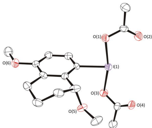
Figure 1: X-ray structures of iodine(III) reagent 8a . Hydrogen atoms are omitted for clarity. Thermal ellipsoids are shown at 50% probability.
