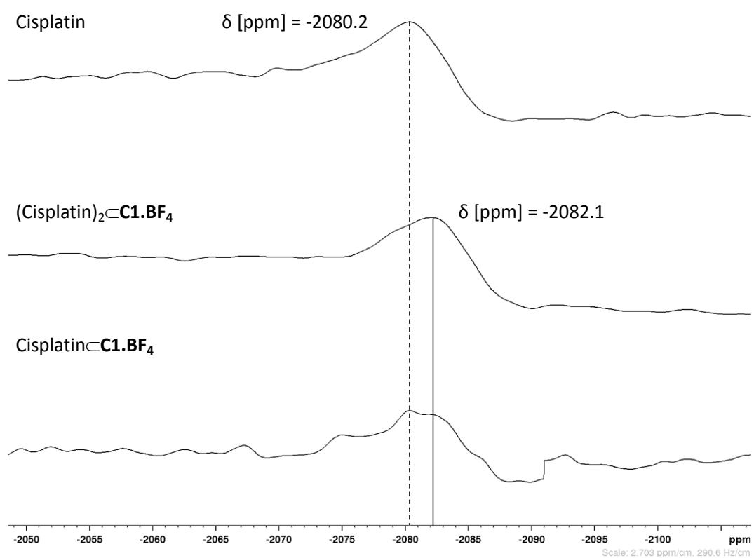
Figure 3 - Stacked 195 Pt NMR spectra in DMF of: (top) cisplatin ( \delta [ppm] = -2080.2); (middle) C1.BF 4 + 2 equiv. of cisplatin ( \delta [ppm] = -2082.1); (bottom) C1.BF 4 + 1 equiv. of cisplatin ( \delta [ppm] = -2082.1).
