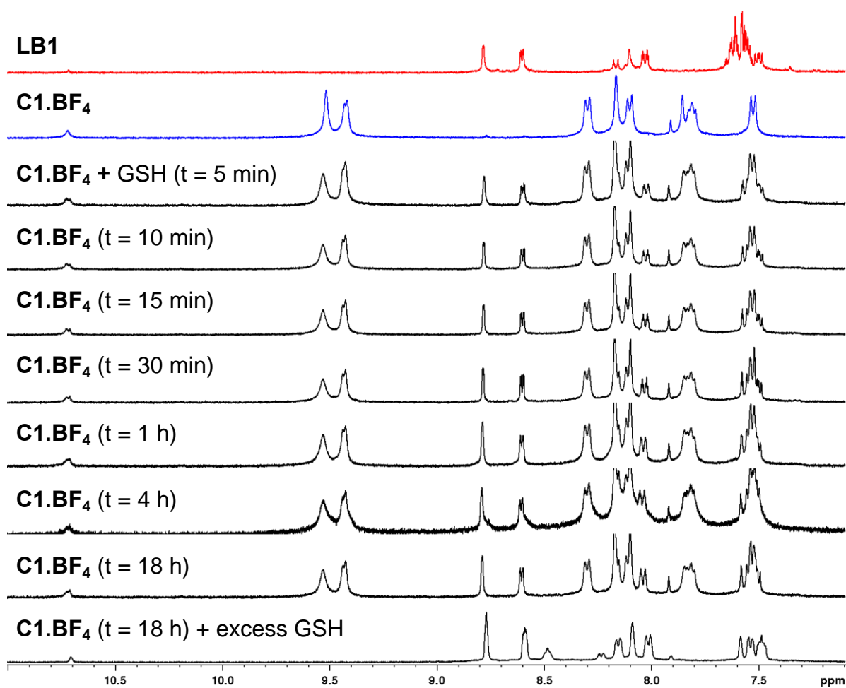
Figure 2. Stacked 1 H NMR spectra of ligand LB1 (top) and of the corresponding metallacage C1.BF 4 (second trace from top) in 9:1 ratio of DMSO- d 6 : D 2 O, in the presence of 2 mM glutathione over time. A further addition of excess GSH was performed after 18 h to achieve complete cage dissociation (bottom spectrum).
