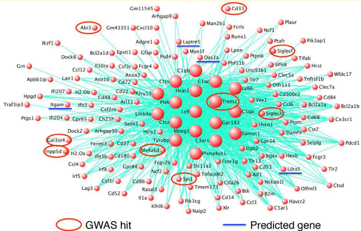
Figure 1 An innate immune network of genes expressed by amyloid-responsive microglia, featuring several orthologues of established GWAS genes associated with Alzheimer's disease, predicts the importance of four new risk genes that may influence the risk of developing Alzheimer's disease. Network plot using VisANT reveals key drivers of an innate immune module from RNA-seq derived gene expression from the hippocampus of wild-type and amyloid mice. Red circles show orthologues of established GWAS genes associated with Alzheimer's disease including Trem2 , Abi3 , Cd33 and Spi1 /PU.1. Blue underline shows gene orthologues predicted to confer altered risk of Alzheimer's disease by overlapping a gene co-expression network present in mouse microglia that show a strong response to amyloid in transgenic mice with individual human genes significantly associated with Alzheimer's disease by analysing combinations of adjacent SNPs (see Materials and methods section; Escott-Price et al., 2014 ). Genes shown in this network are transcribed and co-expressed in amyloid-responsive microglia. Larger red spheres represent 'hub' genes, those showing the greatest number of connections to other genes in the network, and include Trem2 , Tyrobpb , Lilrb4a , P2ry13 , Ctss , Ctsz , Mpeg1 and Plek , which are likely to play important roles in driving microglial function.
