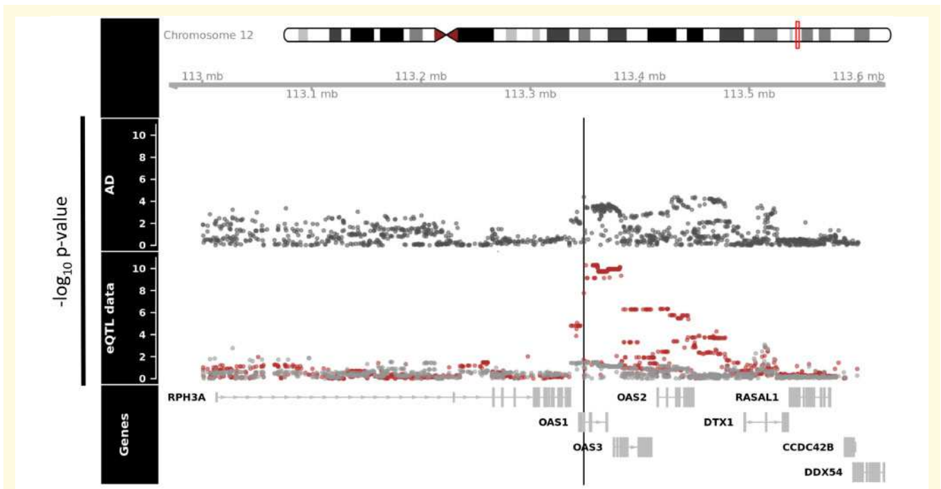
Figure 2 Colocalization of Alzheimer's disease GWAS loci with eQTLs derived from baseline and stimulated iPSC-derived macrophages. Colocalization of Alzheimer's disease loci and eQTLs targeting OAS1 in baseline and stimulated states (interferon- \gamma and Salmonella, 18 and 5 h, respectively). In the eQTL panels, grey and red data points represent macrophages at baseline or stimulated with both interferon- \gamma and Salmonella, respectively. The eQTL data are from Alasoo et al. (2018) . The best Alzheimer's disease locus in OAS1 from the IGAP data ( Lambert et al., 2013 ) is highlighted with the black line. Numerical results are reported in Supplementary Table 4 .
