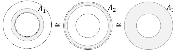
FIG. 3. Annuli A_1 , A_2 and A_3 in the proof of Corollary II.4. Any logical operator on A_3 have two disjoint supports A_1 and A_2 simultaneously, which implies. The isomorphisms from the algebras on smaller regions to the algebra on A_3 are established by the natural embedding.
