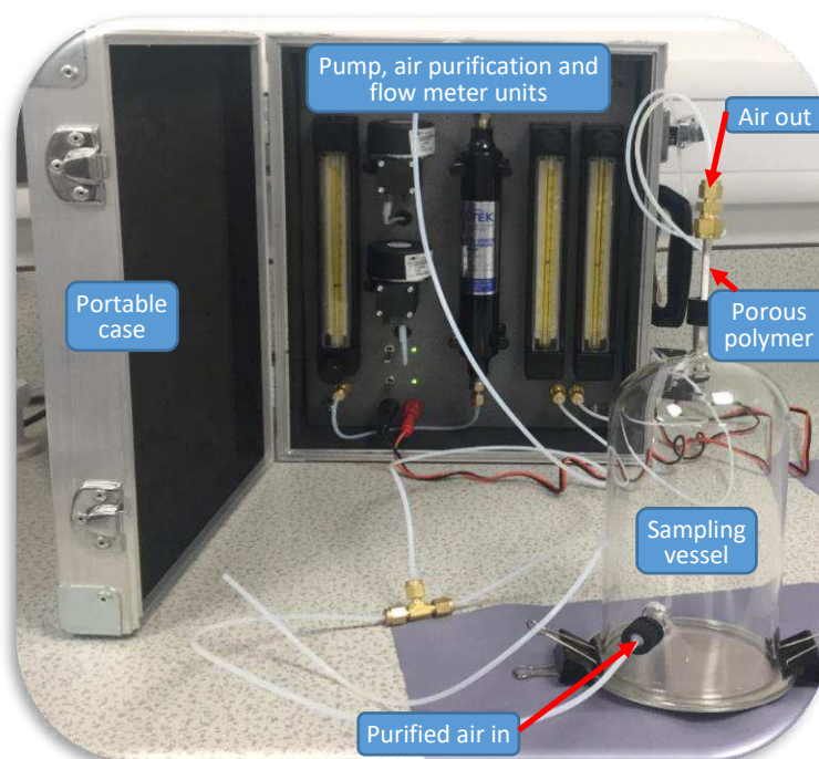
Figure 3 Portable apparatus for entrainment of volatiles from over biological samples, under positive pressure of purified air, by absorption on porous polymer. (Courtesy Irene Castellan, Cardiff University)
