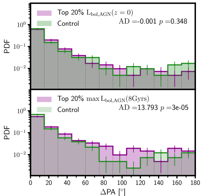
Figure 3. Probability density function of kinematic misalignment as defined by \Delta\text{PA} at z = 0 for low mass galaxies ( M_{\text{stel}} < 10^{10.2} M_{\odot} ). In both panels the brightest 20% in L_{\text{bol,AGN}} (purple) compared with a mass matched control (green) is shown. The top panel shows the brightest in L_{\text{bol,AGN}} at z = 0 only, whereas the bottom panel shows those with the brightest peak L_{\text{bol,AGN}} over the last 8 Gyrs. In each panel the Anderson-Darling statistic with a corresponding p-value is shown. We find no statistical difference between the active galaxies and the control for those selected at z = 0 only, whereas we find that those which have been the most luminous over the last 8 Gyrs are distinctly more misaligned.
