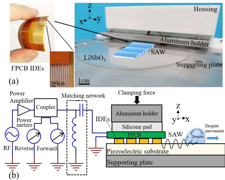
Fig. 1. (a) A photo of the FPCB IDEs and the FPCB-SAW device consisting of a FPCB stacked on a LiNbO 3 substrate. (b) The assembly diagram of the SAW generation on the FPCB-SAW device and its driving circuitry.
