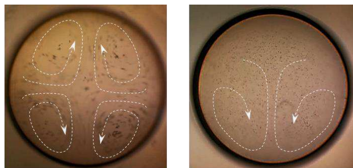
Fig. 5. Acoustic streaming produced by the FPCB-SAW device. (a) Four microsphere micro-vortices are produced within a droplet with low viscosity, the input power is 22 dBm. (b) Two microsphere micro-vortices are produced within a droplet with high viscosity, the input power is 25 dBm
