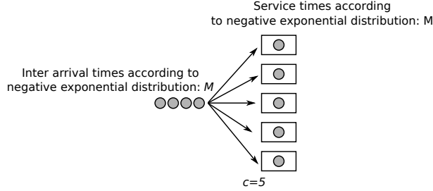
Figure 9: Pictorial representation of an M/M/c queue.
