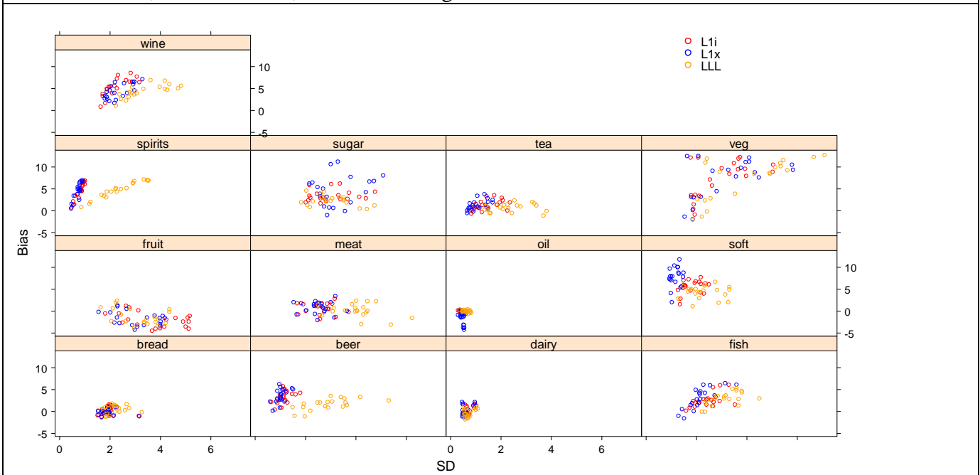
Figure 5 Plots of Bias vs. SD by Sampling Scheme (colour-coded) for different COICOP groups SS-L1i= Red , SS-L1x= Blue, SS-LLL= Orange
