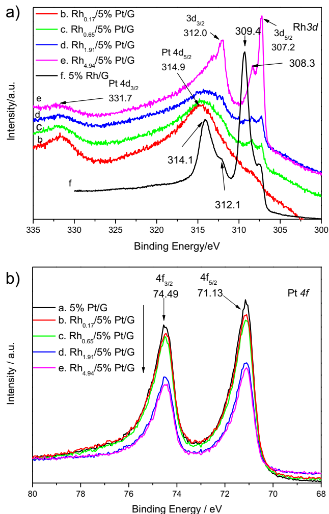
Fig. 3. X-ray photoelectron spectra of (a)—Rh 3d and (b)—Pt 4f regions for fresh Rh_x/5\% Pt/G. The values of x are: a. 0.00, b. 0.17, c. 0.65, d. 1.91, and e. 4.94. In (a) curve f. corresponds to a 5% Rh/G catalyst.
