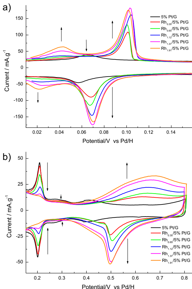
Fig. 1. (a) and (b) are expanded CV profiles of fresh Rh_x/5\% Pt/G for 0 < x < 2 monolayer equivalents. Test solution: 0.5\text{ M H}_2\text{SO}_4 . Sweep rate: 10\text{ mV}\cdot\text{s}^{-1} .
