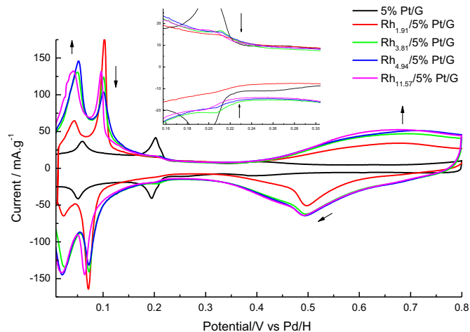
Fig. 2. CV profiles of fresh Rh_x/5\% Pt/G ( 1.9 < x < 12 monolayer equivalents). The insert is the expansion of the Pt(100) \times (111) step H UPD region. Test electrolyte: 0.5\text{ M H}_2\text{SO}_4 . Sweep rate: 10\text{ mV}\cdot\text{s}^{-1} .
