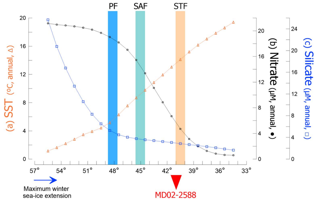
Figure 2. Present-day, annually averaged latitudinal values of (a) SST (°C, light brown line), (b) nitrate ( \mu\text{M} , black line), and (c) silicate ( \mu\text{M} , blue line) along 25°E in the Southern Ocean and the Indian-Atlantic Ocean gateway between 57° and 33°S off the southern tip of South Africa (LEVITUS94, http://iridl.ldeo.columbia.edu/SOURCES/LEVITUS94/ ). The blue arrow indicates the maximal present-day extension of the winter Antarctic sea ice cover between 23° and 27°E. The inverted red triangle shows the location of site MD02-2588. References: SAF: Sub-Antarctic Front (light blue); STF: Subtropical Front (light orange bar); PF: Polar Front (dark blue bar) [after Peterson and Stramma, 1991; Orsi et al., 1995].
