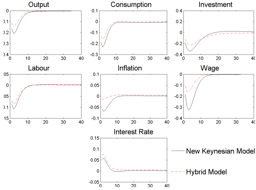
Figure 10: IRFs of Monetary Shock ( \eta_r )
