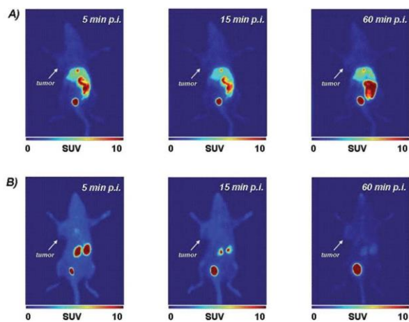
Fig. 4 PET images (maximum intensity projection) of ^{64}\text{Cu} ]Cu–CryptTM (A) and for ^{64}\text{Cu} ]Cu–DiAmSar (B) at selected time points after single intravenous injection (5 MBq for each complex) into EMT-6 tumor-bearing BALB/c mice.
