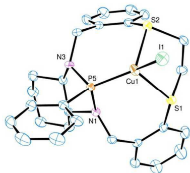
Figure 2 Ortep view of the molecular structure of [\text{Cu}(\mathbf{2})\text{I}] , 4 . Hydrogen atoms and lattice solvent are omitted for clarity. Selected bond lengths (Å) and angles ( ^\circ ): Cu1-P5 2.1729(12); Cu1-S1 2.4990(13); Cu1-S2 2.3563(12); Cu1-I1 2.5396(7); N1-P5-N3 93.20(19); P5-Cu1-S1 103.49(4); P5-Cu1-S2 109.95(5); P5-Cu1-I1 135.65(4); S1-Cu1-S2 90.81(4); S1-Cu1-I1 106.45(4); S2-Cu1-I1 101.61(4).
