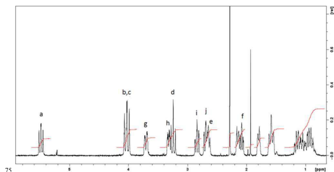
Figure 3 Section of the ^1\text{H} NMR spectrum of [\text{Mo}(\text{CO})_3(\mathbf{2})] , 5 . The peaks labelled a-d are those of the benzylic hydrogens alpha to the nitrogens and those labelled e,f are the methine hydrogens. The g-j resonances are for the hydrogens of the dimethylene bridge between the sulphur atoms.
