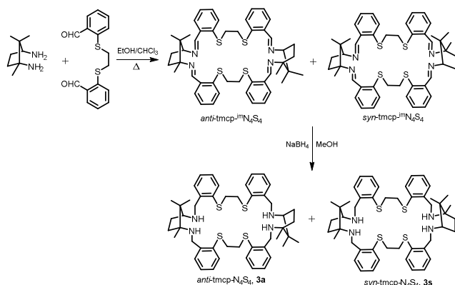
Scheme 2 Synthesis of syn - and anti -tmcp- N_4S_4
