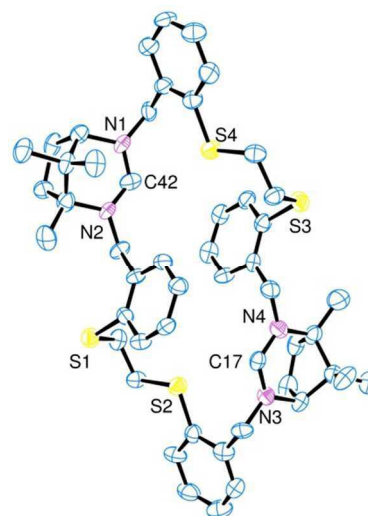
Figure 4 Ortep view of the molecular structure of the syn -[tmcp-diamidS 4 ] dication. Hydrogen atoms, counterions and lattice solvent are omitted for clarity. Selected bond lengths (Å) and angles(°): C17-N4 1.307(16); C17-N3 1.304(14); C42-N1 1.314(14); C42-N2 1.304(16); N1-C42-N2 123.4(12); N3-C17-N4 123.8(11).
