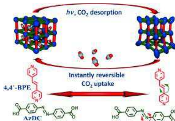
Fig. 8 Reversible photoinduced \text{CO}_2 uptake in MOF Zn-(AzDC)(4,4'-BPE) 0.5 . Reproduced with permission from ref 97. Copyright 2013 Wiley-VCH.
