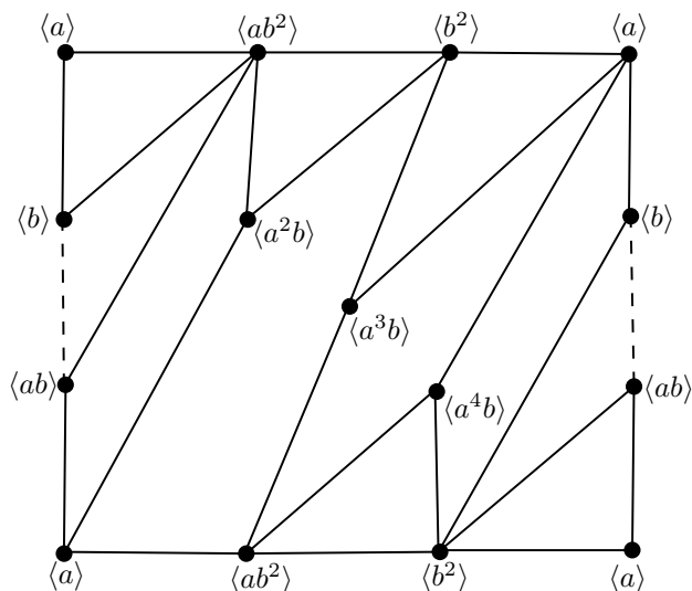
Figure 4: A toroidal embedding of \Gamma(\mathbb{Z}_5 \times \mathbb{Z}_4) .
