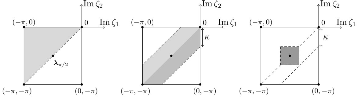
Figure 1: The two-dimensional bases -\mathcal{G}_2 (left), -\mathcal{B}_2(\kappa) (middle) and \boldsymbol{\lambda}_{\pi/2} + \mathcal{C}_2(\kappa) (right).
