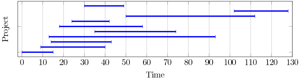
(b) Both objectives are enabled, that is, the primary objective is the TPD – minimising the sum of completion times of projects. TPC = 654, TMS = 128.
