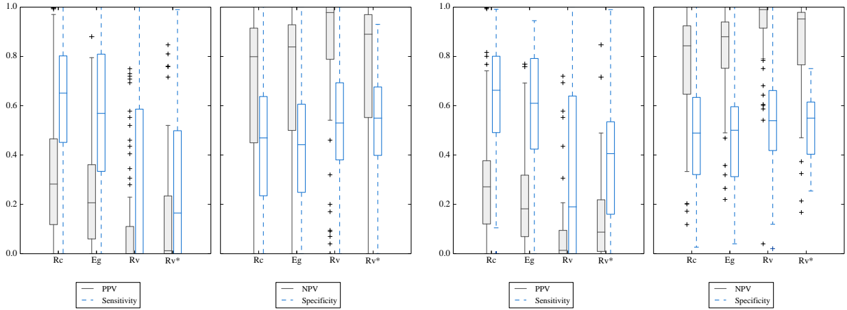
(a) All users. Reachability (N=92), Engage-ability(N=92), Recep- (b) Users with >10 notifications. Reachability (N=63), Engage- tivity (not-in-use: N=92, in-use: N=83). ability(N=63), Receptivity (not-in-use: N=63, in-use: N=41).
