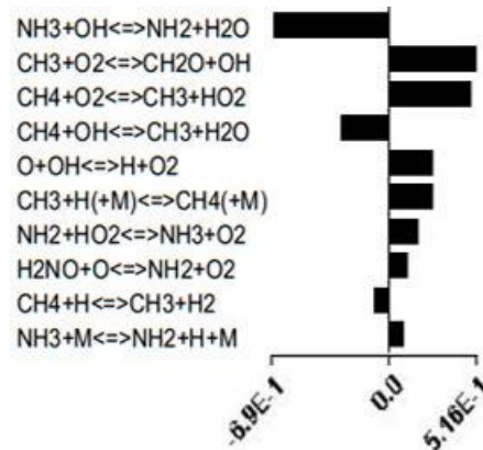
Fig. 9. OH sensitivity using ÅA mechanism.
