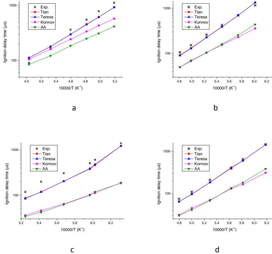
Fig. 3. Performance of different mechanisms with respect to ignition delay times of NH 3 mixtures. a) 1.4 atm, E.R. = 0.5, 99% Ar; b) 11.0 atm, E.R. = 1.0, 99% Ar; c) 30.0 atm, E.R. = 2.0, 99% Ar; d) 11.0 atm, E.R. = 1.0, 98% Ar. Experiments as in [14].
