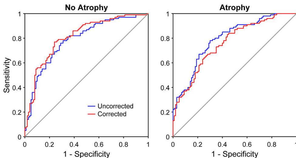
Figure 6. Receiver operating characteristic (ROC) curves illustrating the impact of correcting GABA measurements for tissue-dependent concentration differences in hypothetical diseased ( D^+ ) and non-diseased ( D^- ) cohorts. Two scenarios were simulated: one where atrophy was not present in D^+ and one where atrophy was present in D^+ . The uncorrected ROC curves (blue) in both scenarios had an area under the curve (AUC) of \sim 0.80 . When both cohorts exhibited similar mean t_{GM} values (no atrophy scenario), the tissue correction led to a small increase in the AUC (red ROC curve). When D^+ had a lower mean t_{GM} (atrophy scenario), the tissue correction led to a decrease in the AUC.
