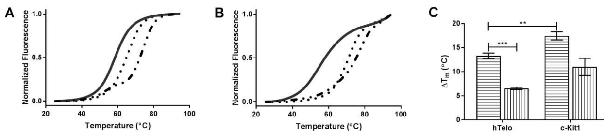
Figure 3. Representative FRET melting profiles of a 0.2 \mu\text{M} hTelo (A) and C-KIT1 (B) G-quadruplex DNA solutions in 60 mM potassium cacodylate buffer in absence (black solid lines), and in presence of 1 \mu\text{M} of AuTMX 2 (dotted lines) and AuTMX-I (dashed lines). C) \Delta T_m of hTelo and C-KIT1 G4s in the presence of AuTMX 2 (horizontal lines) and AuTMX-I (vertical lines). Data is shown as mean \pm SEM of three independent experiments; ** p < 0.005 , *** p < 0.001 . Results for AuTMX-I hTelo vs C-KIT1 are significantly different (significance not shown in the plot), * p < 0.05 .
