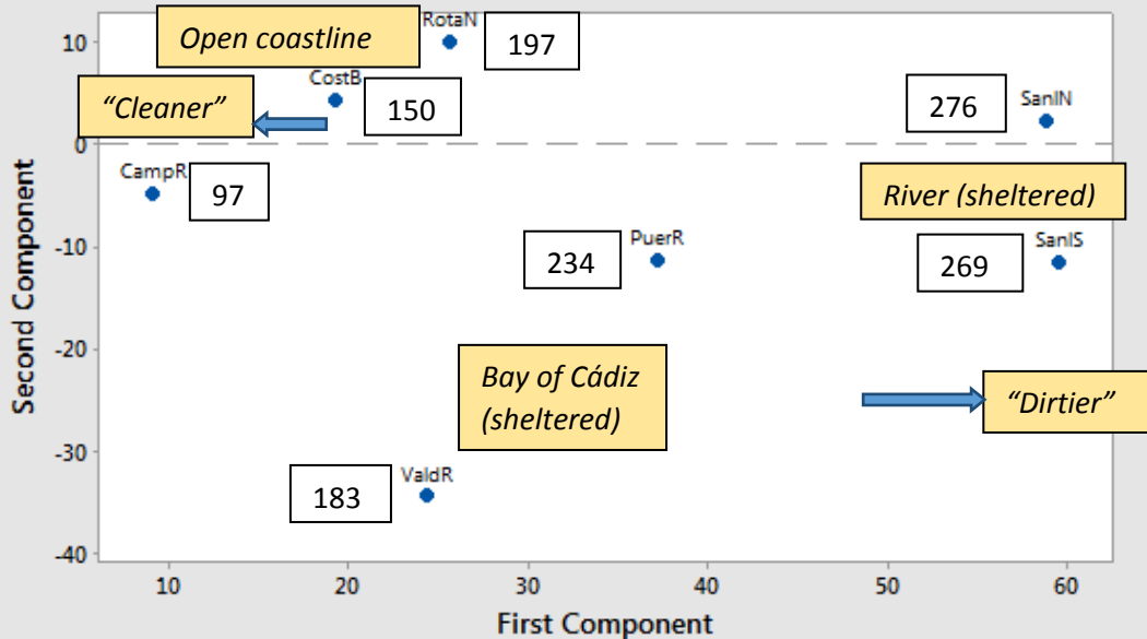
Score Plot of CL04, ..., YYXX Cadiz: 7 sites, 49 categ. (Covariance, non-stand.)
